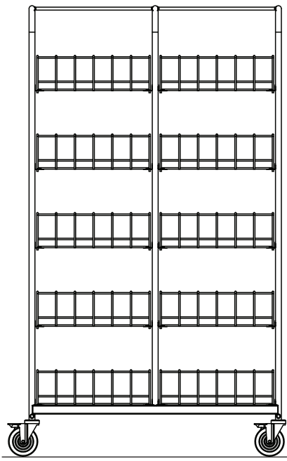
Front Elevation Model USR120
